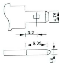
Terminal Type (mm)
