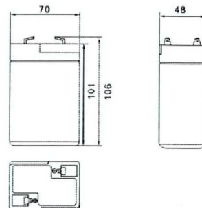
Outer dimensions (mm)
